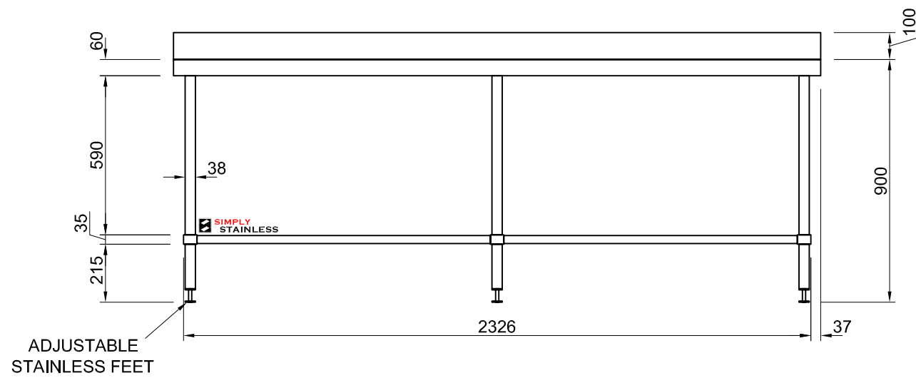
FRONT ELEVATION
