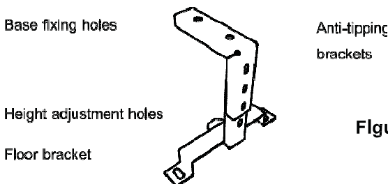
Figure 1 - Anti-tipping Bracket
