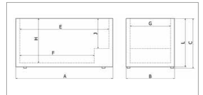
Dimensions according to technical datas below
