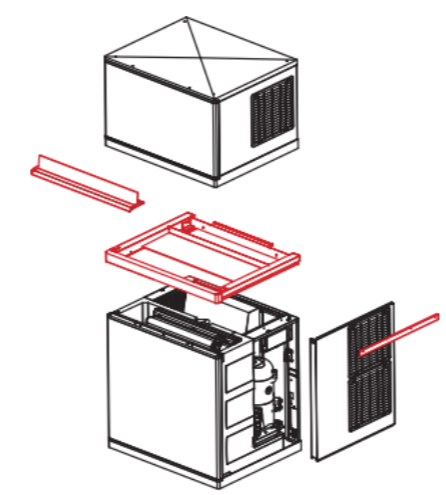
Optional Union Kit For Stacking 2 x Ice Machines
